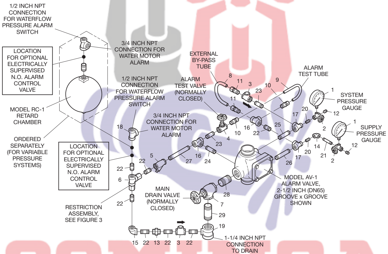
FIGURE 4 (1 OF 3) VERTICAL CLOSED DRAIN TRIM – STANDARD ORDER FOR 2-1/2 INCH (DN65) MODEL AV-1-300 ALARM CHECK VALVES (P/N 52-204-4-950)
