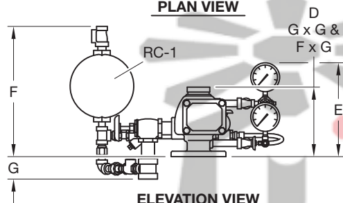
ELEVATION VIEW
