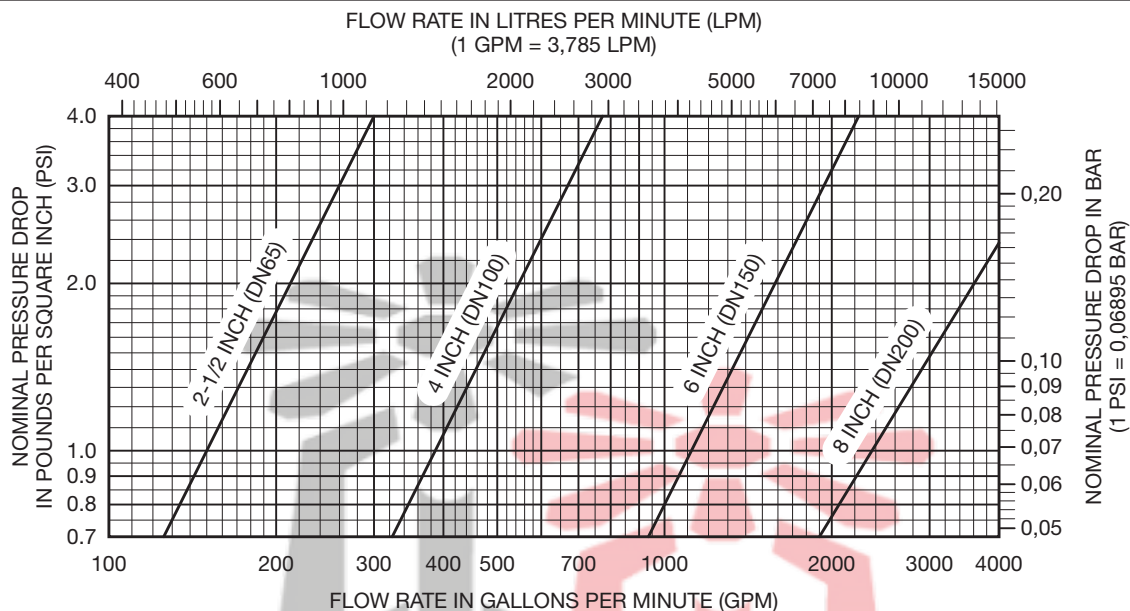
GRAPH A MODEL AV-1-300 ALARM CHECK VALVE NOMINAL PRESSURE LOSS VERSUS FLOW
