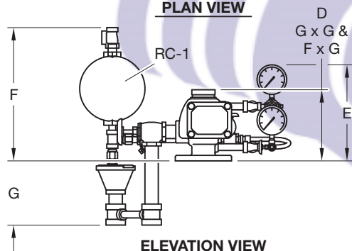
FIGURE 7 (1 OF 3) INSTALLATION DIMENSIONS FOR 2-1/2 INCH (DN65) MODEL AV-1-300 ALARM CHECK VALVES
