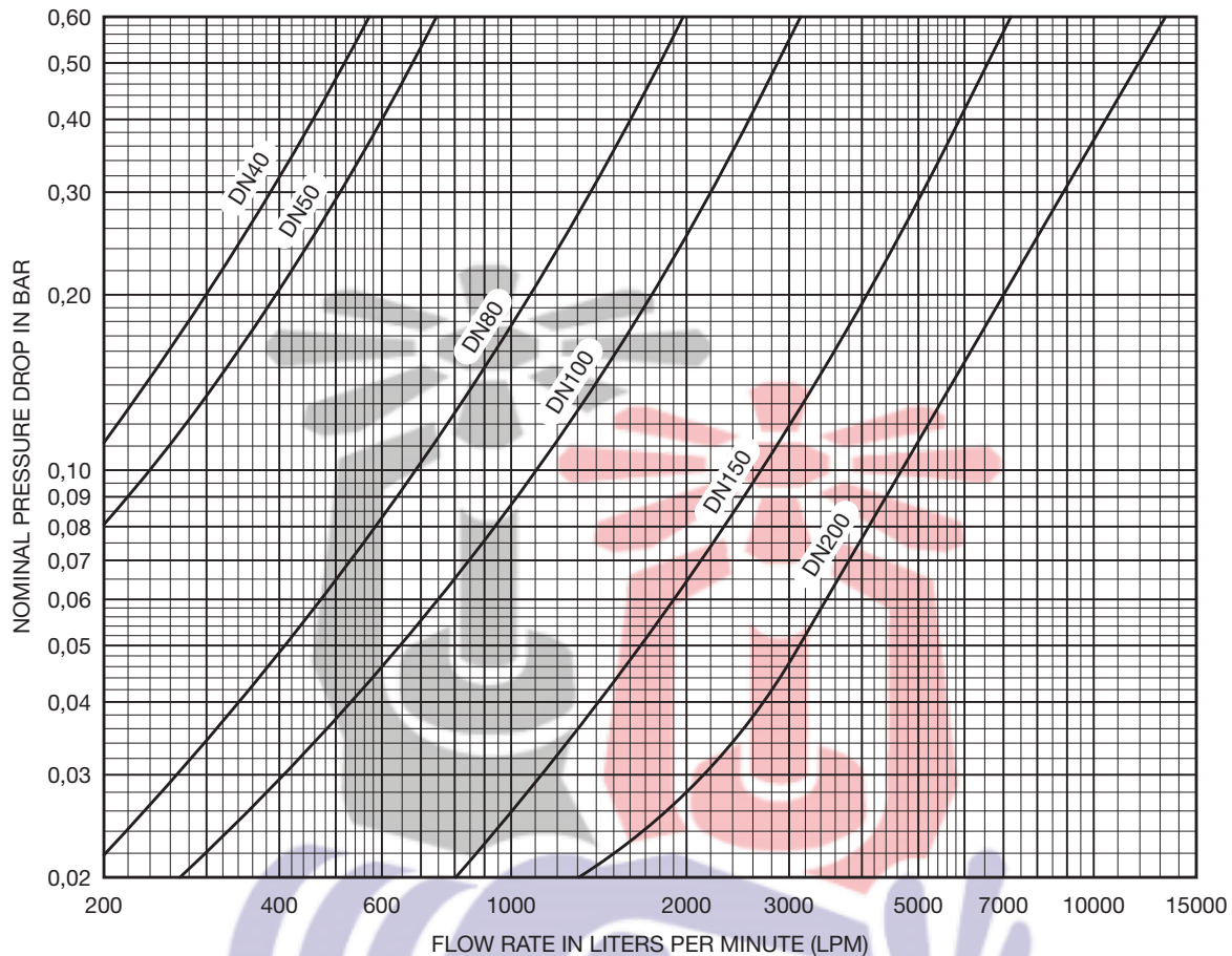
GRAPH A DN40 THRU DN200 DV-5 VALVE AND MODEL CV-1FR VALVE NOMINAL PRESSURE LOSS VERSUS FLOW
