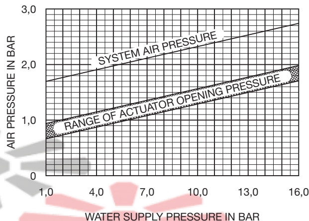
GRAPH B AIR (NITROGEN) MINIMUM SUPPLY PRESSURE (VdS) 3 BAR PRESSURE REQUIREMENT
